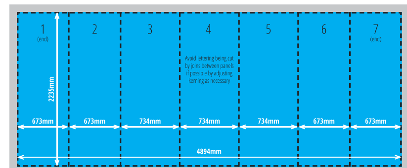
5x3 Hybrid Panel Sizes
