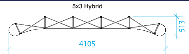
5x3 Hybrid Panel Sizes
