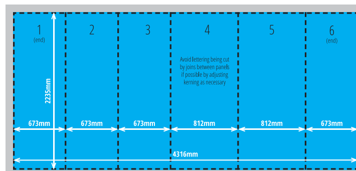
4x3 Hybrid Panel Sizes
