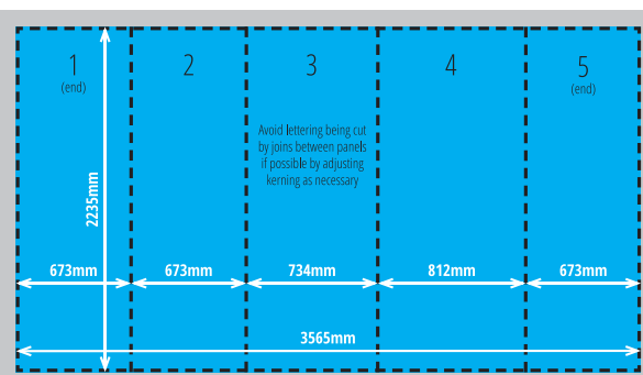
3x3 Hybrid Panel Sizes
