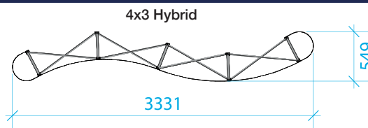
4x3 Hybrid Panel Sizes
