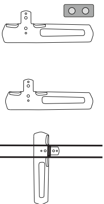
Single-sided
