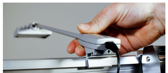
11 Mount the lights.
