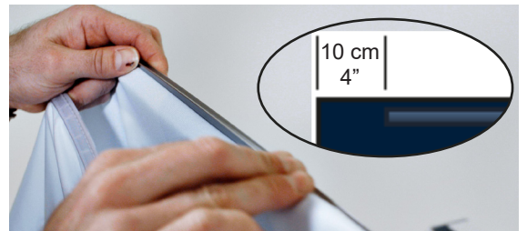
9 Press the plastic strip into the upper track of the profiles. Leave 10 cm/4 inches on each side for the fabric end holders.
